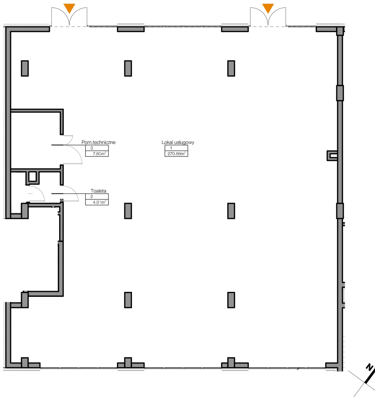
SCHEMAT PARTERU
